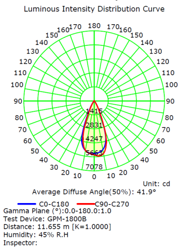
CYN 40R WS25 25W SD36 VB 927K (36° Beam Angle)
