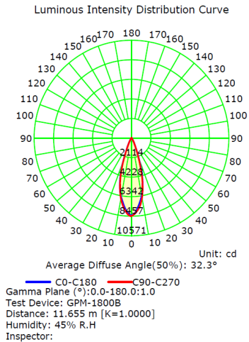
CYN 40R WS25 25W SD24 VB 927K (24° Beam Angle)
