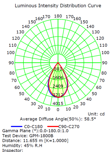
CYN 40R WS25 25W SD50 VB 927K (50° Beam Angle)
